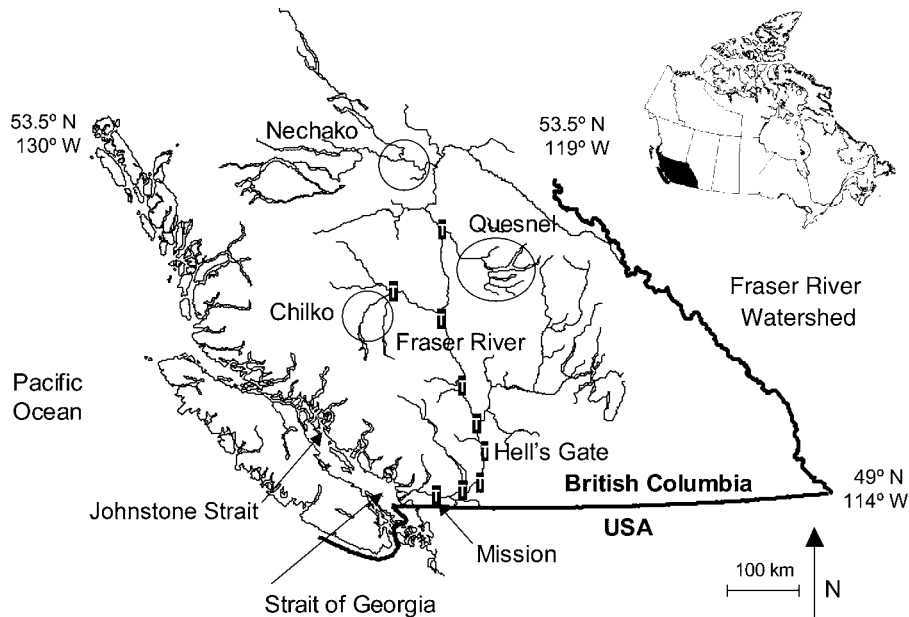
FIG. 1. Map of Canada with an inset of the Fraser River Watershed of British Columbia. Key locations are identified on the map including the river-entry telemetry station at Mission. Additional telemetry stations are indicated by the "T" in black boxes. Natal spawning watersheds and general terminal spawning locations are circled.
